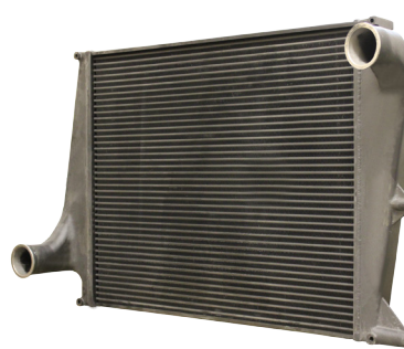
Grayson Part No: AC-5032-000 O.E Number: 20735696/1665242 Description: FH12/16 - FM9/12/16 Dimensions: Length: 760mm Width: 885mm Depth: 47mm
