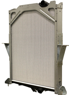
Grayson Part No: RR-5120-000 O.E Number: 20460178/20482258 Description: FM9/11/12 Dimensions: Length: 900mm Width: 740mm Depth: 48mm
