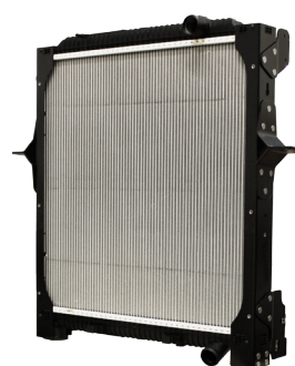
Grayson Part No: RR-3363-000 O.E Number: 20810099/7420810095 Description: FE Dimensions: Length: 735mm Width: 705mm Depth: 43mm
