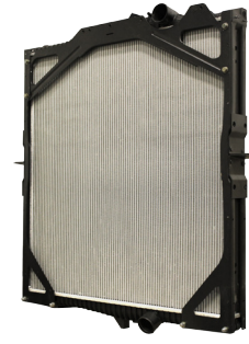
Grayson Part No: RR-5044-000 O.E Number: 1676635/1676435 Description: FH12/16 - FM12 Dimensions: Length: 900mm Width: 870mm Depth: 48mm
